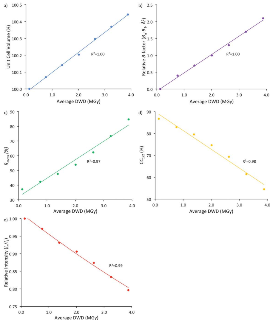
Figure 3 Radiation damage metrics and data quality indicators for the seven consecutive complete data sets as a function of dose, with linear fits shown for (a)–(d) and an exponential fit for (e). (a) The unit cell volume expands with increasing absorbed dose, as does (b) the relative B -factor and (c) R_{\text{meas}} , but (d) \text{CC}_{1/2} and (e) the relative diffraction intensity decrease with dose.
