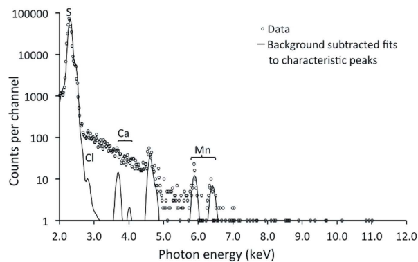
Figure 2 Spectrum of the elemental analysis of XI measured with microPIXE showing the presence of manganese, calcium, chlorine and sulfur. Note that only elements heavier than magnesium were detected in this experiment. The peak between the Ca and Mn corresponds to twice the sulfur peak energy and is due to pile-up in the Si(Li) X-ray detector of the sulfur signals.
