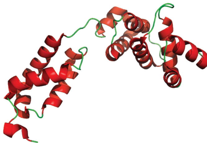
Figure 4 Structure of the N-terminal domain resulting from the harvested crystals (Grant et al. , 2012). Coordinates have been deposited as PDB ID 3t14.
