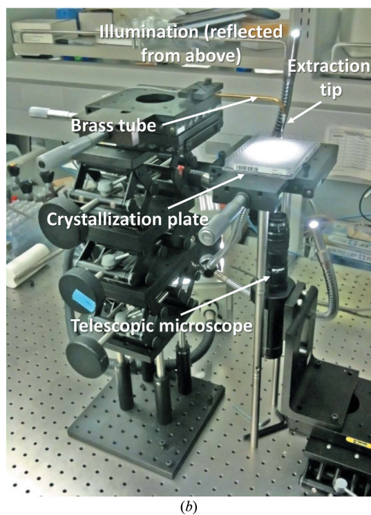
Figure 1 Schematic of the system (a) and a photograph (b) of the actual system. Note that the Hamilton syringe is not visible in (b) and that two sources of illumination are used, reflected illumination from the top and illumination from the bottom. The XY translation stages are not labelled. The brass tube sits on one while the crystallization plate sits on another.
