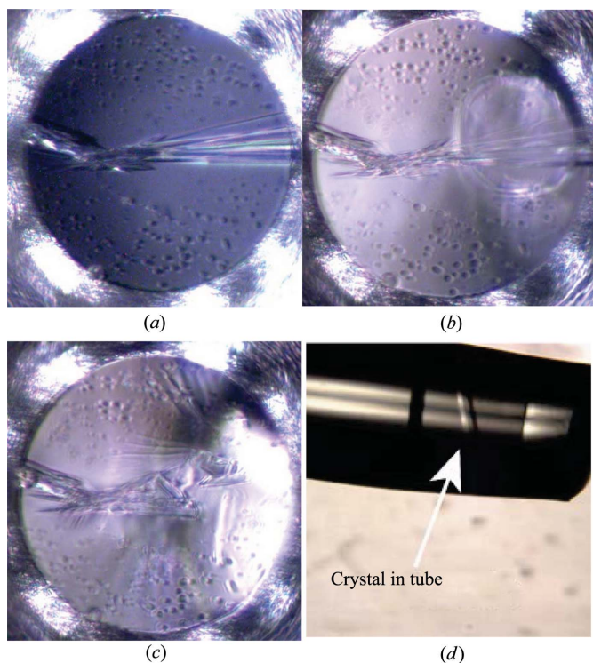
Figure 3 Time sequence monitoring the crystallization drop ( a ) before the polyester tube is inserted, ( b ) as it is inserted and positioned over the crystal, and ( c ) after it is removed and the crystal taken with it. In this case crystals spanned the entire well (0.9 mm in diameter) and the tube was used to separate the crystals and select only a single crystal to mount and subsequently cryocool. In ( d ), the crystal is shown in the polyester extraction tube (0.4 mm diameter) after extraction from the well. Note that the crystal and mother liquor are separated from the mineral oil above (already in the tubing) and below (extracted from the well) which does not mix.
